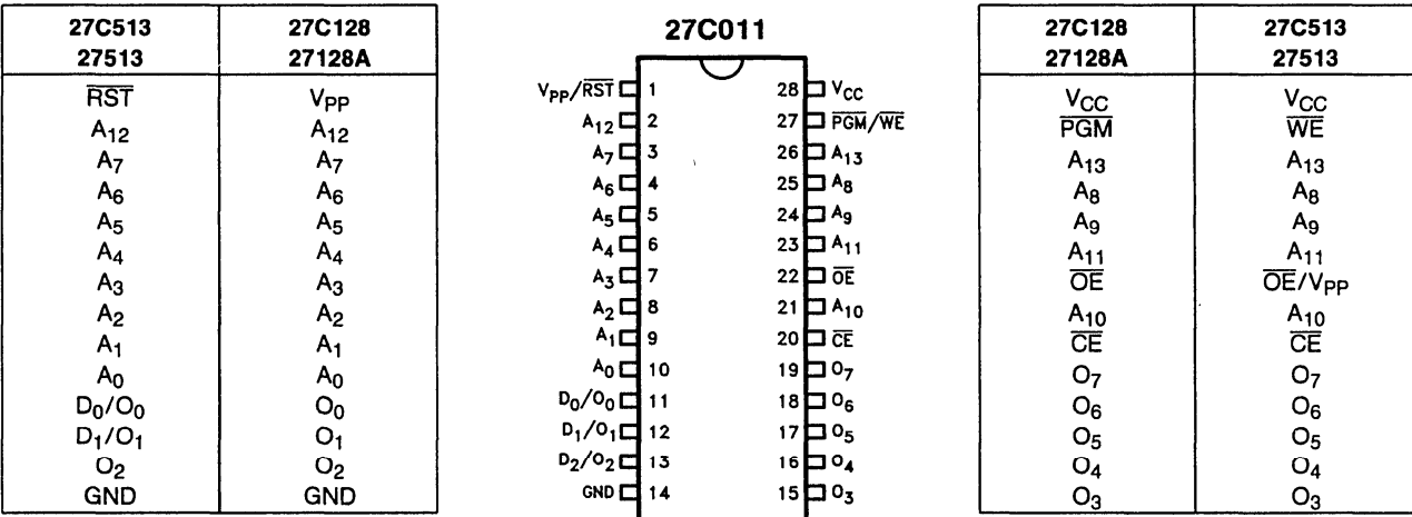
Figure 2. Pin Configuration
