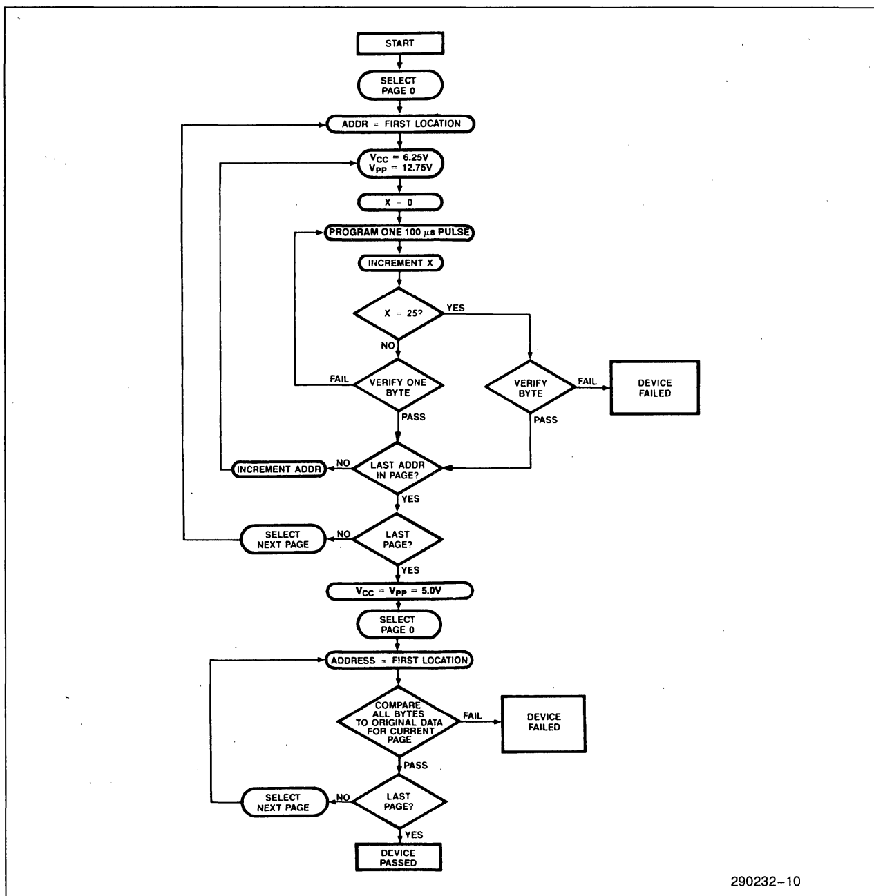
Figure 4. 27C011 Quick-Pulse Programming Flowchart
