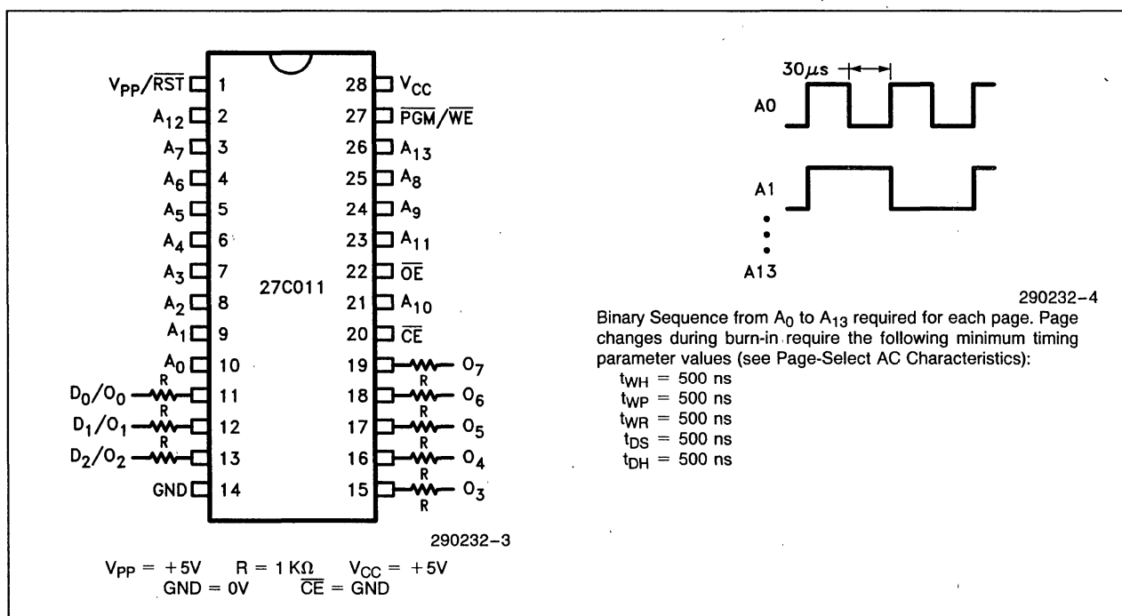
Burn-In Bias and Timing Diagrams
