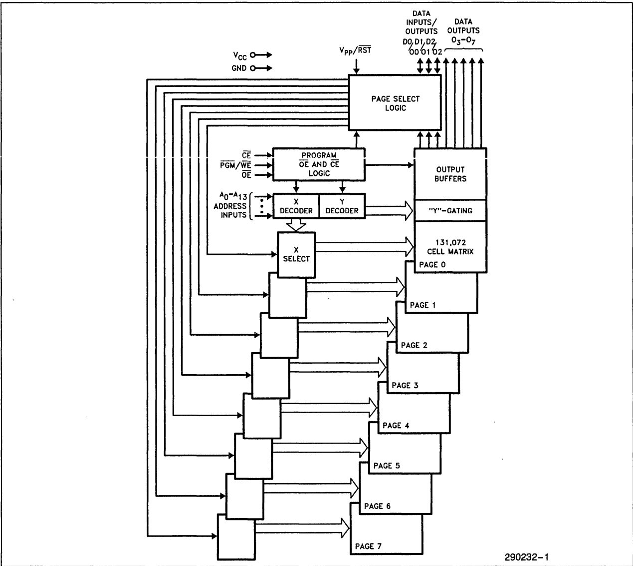
Figure 1. Block Diagram
