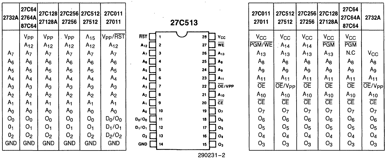
Figure 2. Pin Configuration
