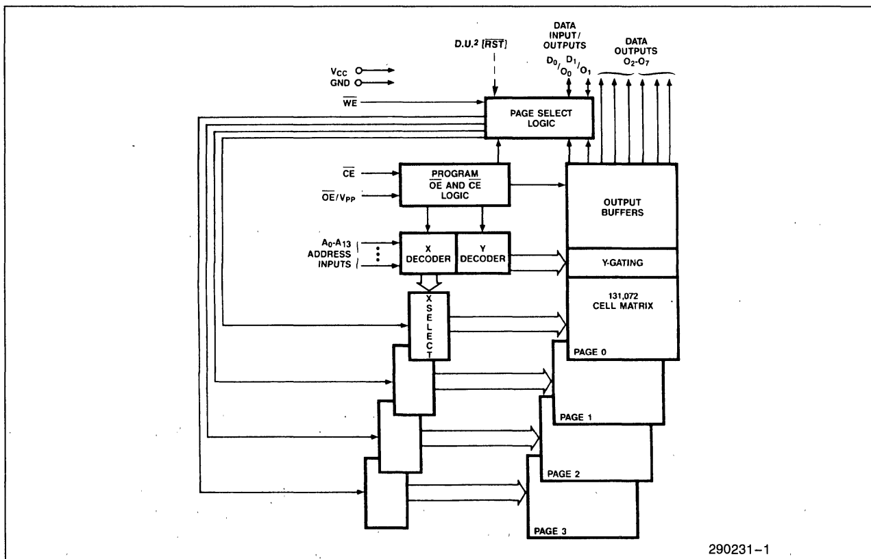
Figure 1. Block Diagram
