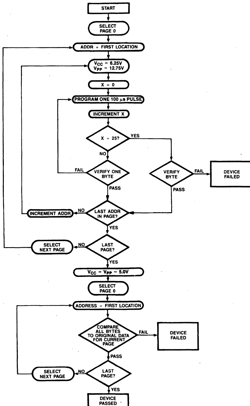
Figure 3. 27C513 Quick-Pulse Programming Flowchart
